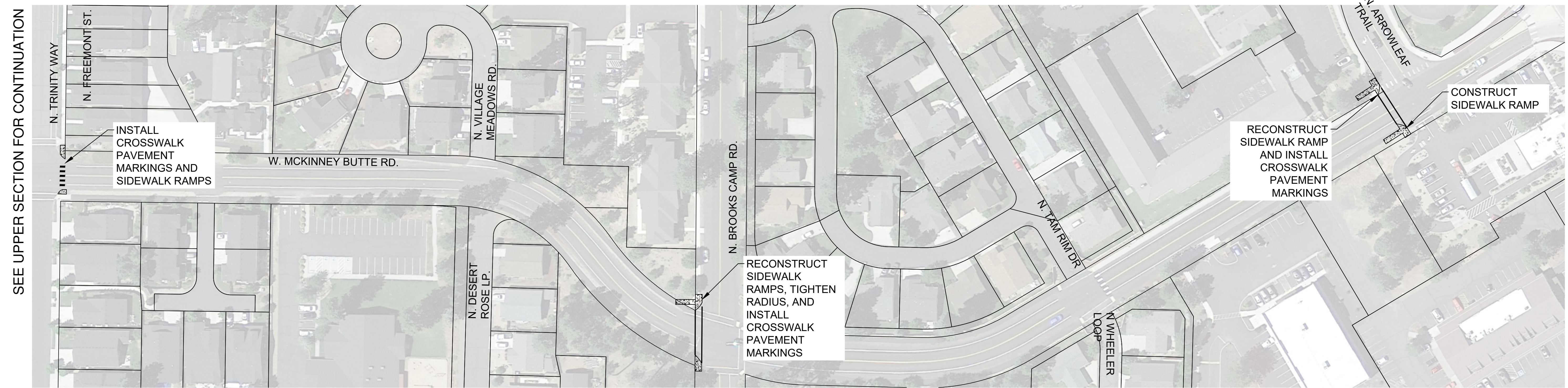
PLAN 2 SCALE: 1"=60' C-1
