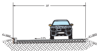
3 ALLEY SECTION M1.4 ALLEY A
